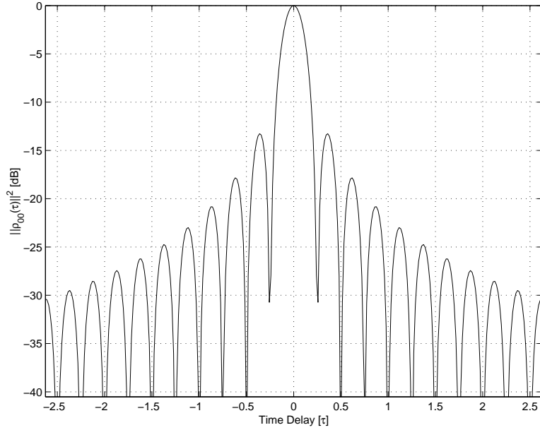
Figure 4.14. Autocorrelation function for a Chebyshev basis with N = 3 and G_D = 0 dB.
