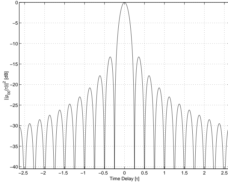
Figure 4.18. Autocorrelation function for a piecewise basis with N = 3 , G_D = 0 dB, and \mathbf{a} = [1 \ 2 \ 4]^T .
