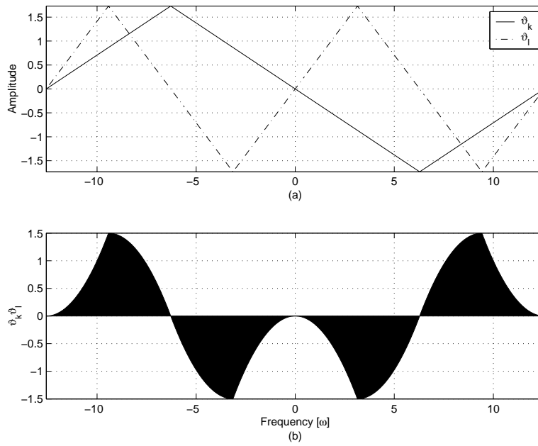
Figure B.2. Orthogonal piecewise functions. \vartheta_k(\omega) and \vartheta_l(\omega) selected such that \max\{a_k, a_l\}/\min\{a_k, a_l\} = 2 , (a), and Area under \vartheta_k(\omega)\vartheta_l(\omega) , (b).
