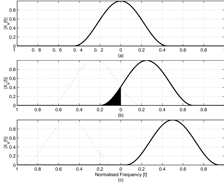
Figure 2.3. Spectral modulation of a bandlimited signal. A bandlimited signal, (a), can be represented using analytic signal notation provided its modulated spectrum, (b), exists in only one hemisphere, (c).
