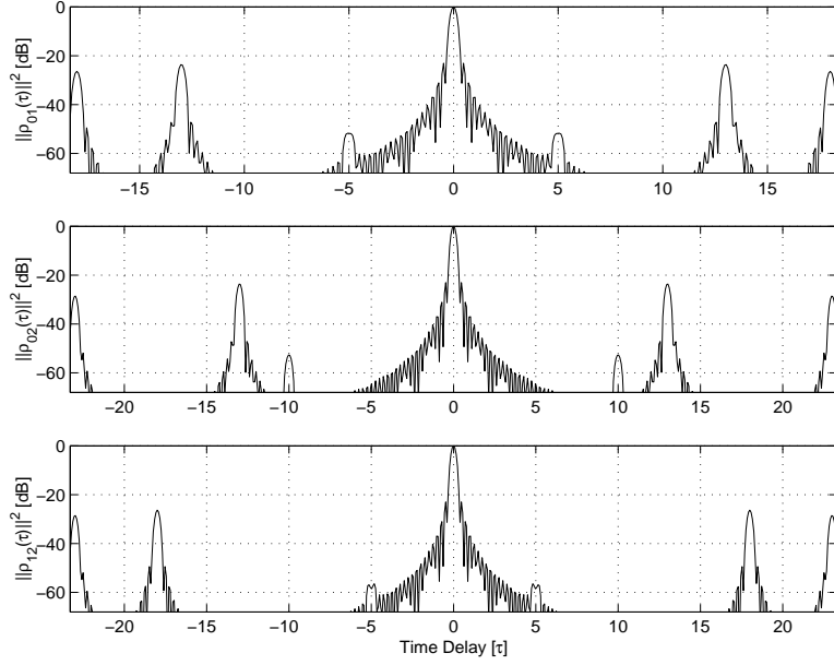
Figure 4.2. Crosscorrelation functions for a sinusoidal basis with N = 3 , G_D = 0 dB, and \mathbf{a} = [13 \ 18 \ 23]^T .
