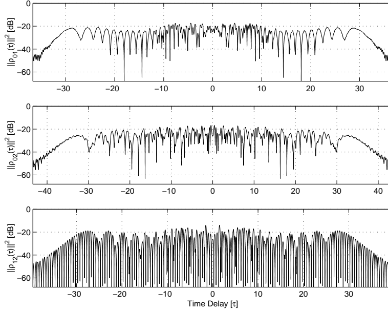
Figure 4.20. Crosscorrelation functions for a piecewise basis with N = 3 , G_D = 20 dB, and \mathbf{a} = [1 \ 2 \ 4]^T .
