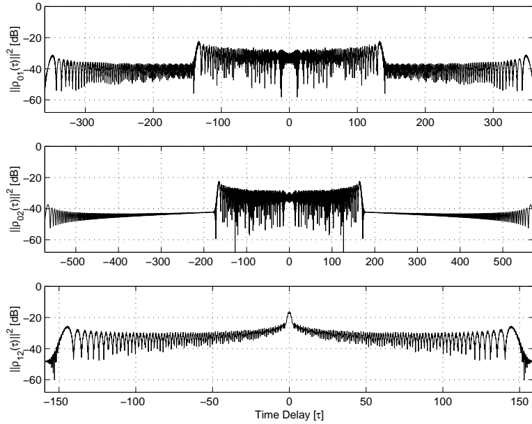
Figure 4.13. Crosscorrelation functions for a polynomial basis with N = 3 and G_D = 40 dB.
